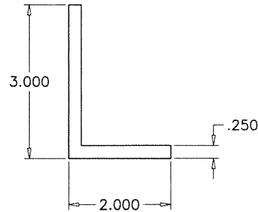
2 INSTALLATION ANGLE
